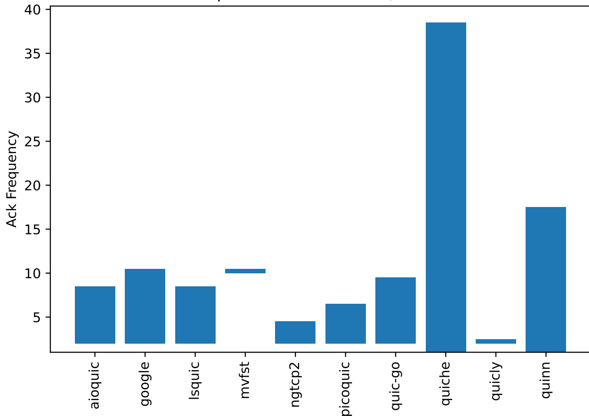
Ack frequencies of different QUIC servers
